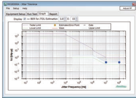
MX183000A High-Speed Serial Data Test Software Measurement Screen
